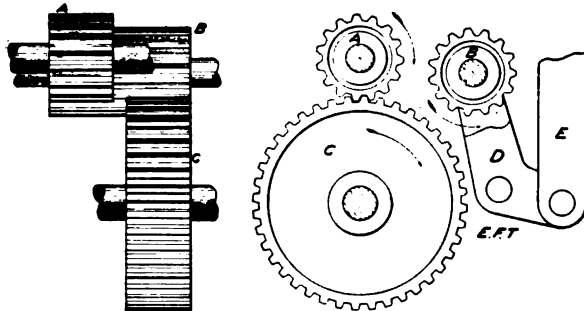
FIG. 350.—Details of the Reverse Gear used on the Daimler-Maybach Carriages. The change speed gear used on these carriages is identical with that used on the Panhard-Levassor, except for the bevel gear reversing arrangement. Instead of using this device, the pulley, A , on the main shaft, is thrown into gear with pulley, C , upon the second shaft, through the spur pinion, B , carried on the bell crank, D , and moved in or out of gear by lever, E . Thus the motion of A is transmitted to C in the reverse direction, although none of the gears on the first and second shafts may be in mesh.
